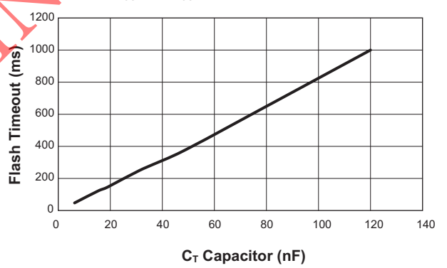
Flash Timeout Delay vs. C_T Capacitor
